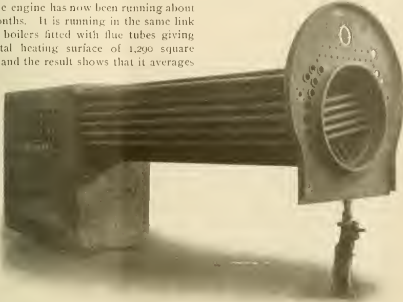
WATER TUBE BOILER WITHOUT SHELL—LONDON & SOUTHWESTERN RAILWAY.
